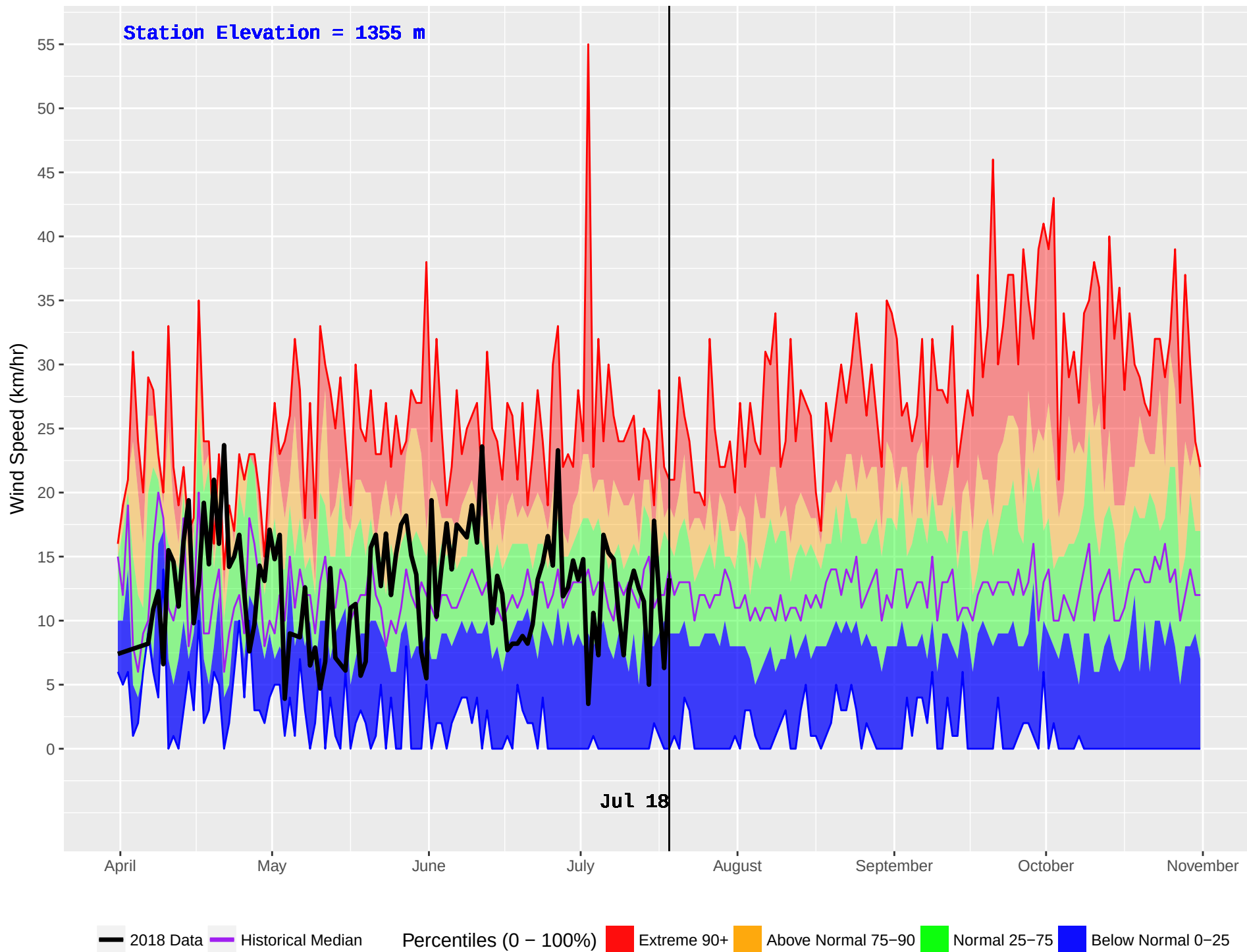
BIG VALLEY (262) : Historical (1987–2016) and Current (2018) Daily Wind Speed
