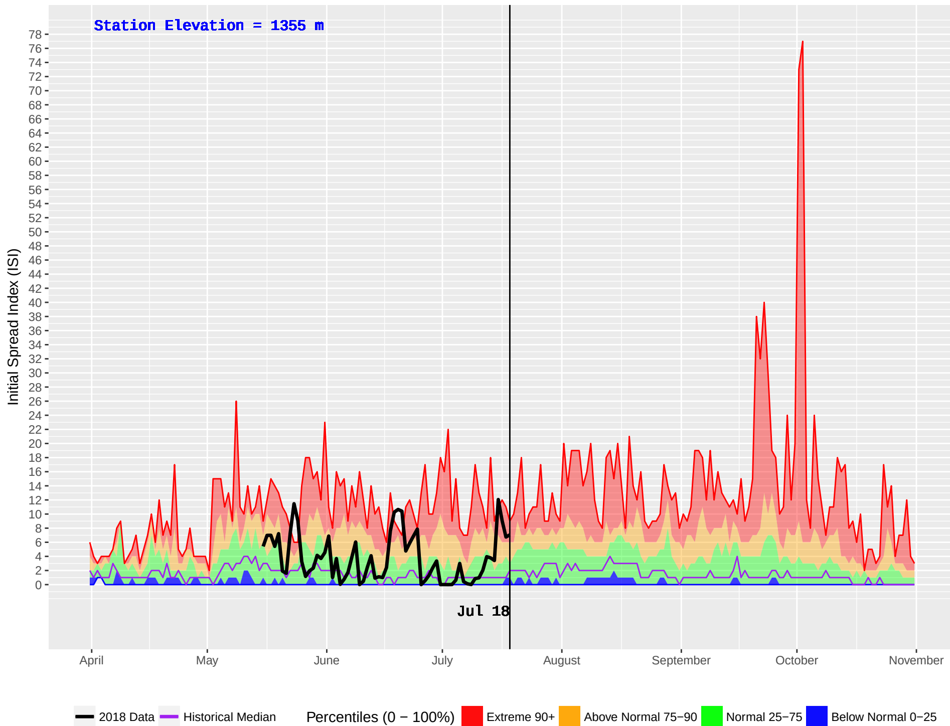
BIG VALLEY (262) : Historical (1987–2016) and Current (2018) Daily Initial Spread Index (ISI)
