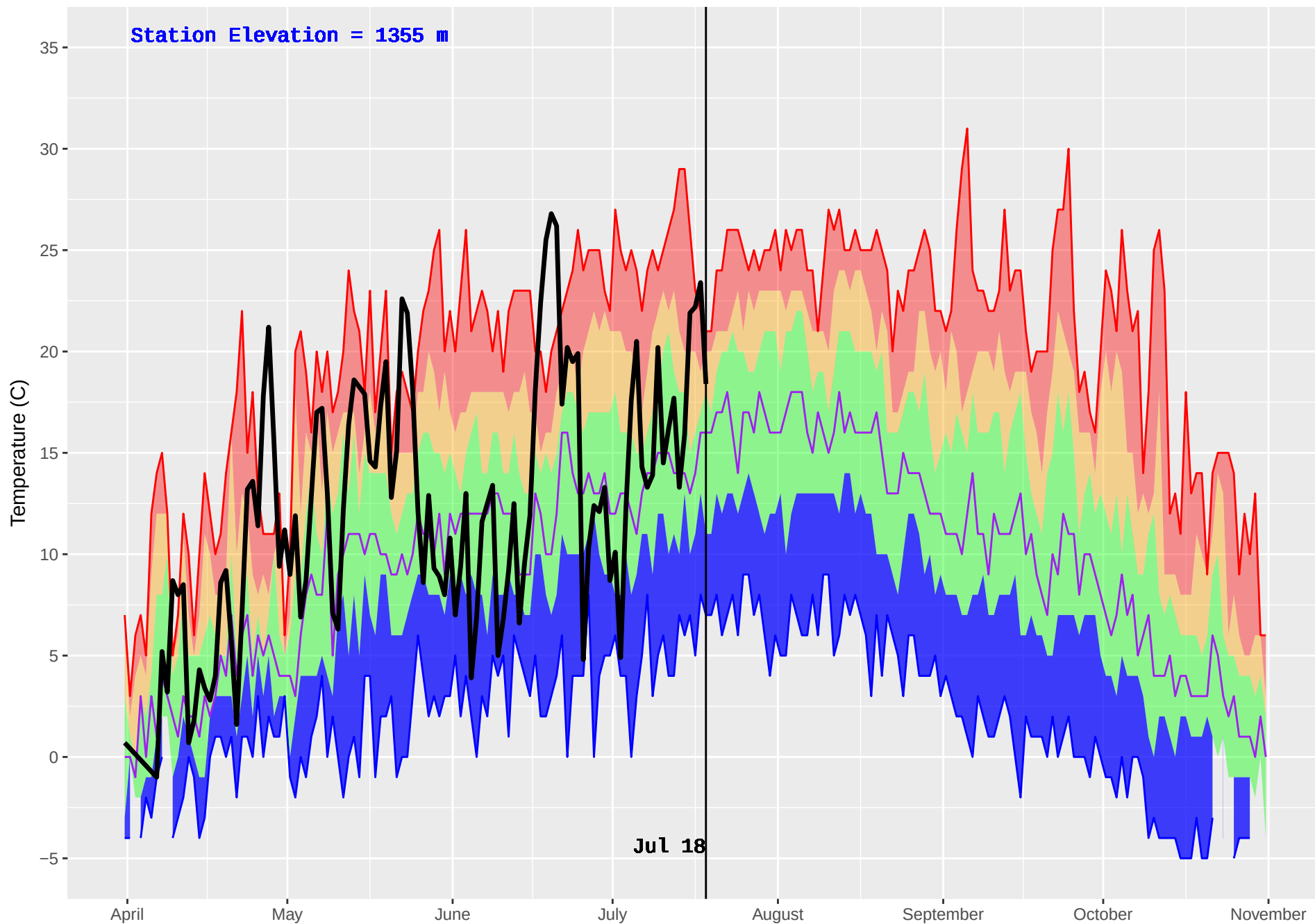
BIG VALLEY (262) : Historical (1987–2016) and Current (2018) Daily Temperature
